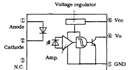
Pin Nos. and internal connection diagram
