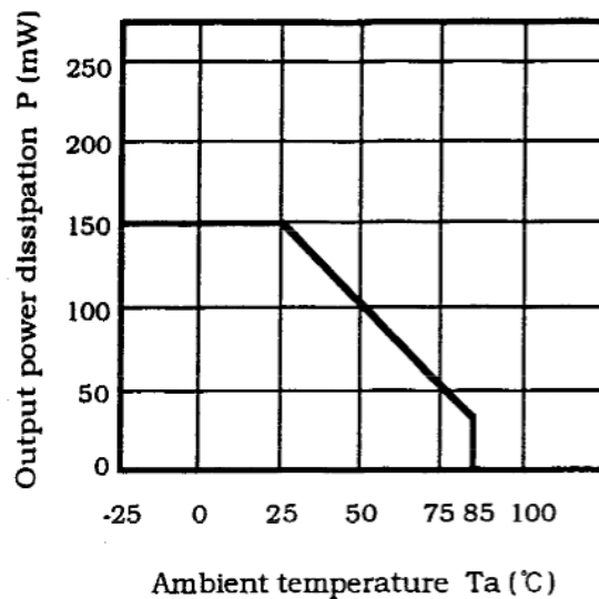
(Fig. 2) Output power dissipation vs. ambient temperature
